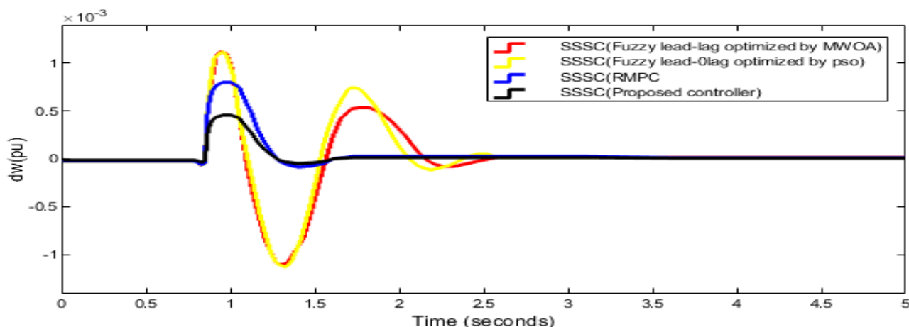
Fig. 7. The changes in the rotor angular velocity over time and based on different controllers , Scenario 2.
