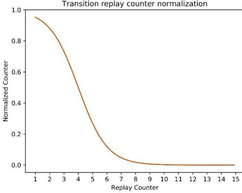
Fig. 1. Normalizing transition replay counter using the Sigmoid function.
