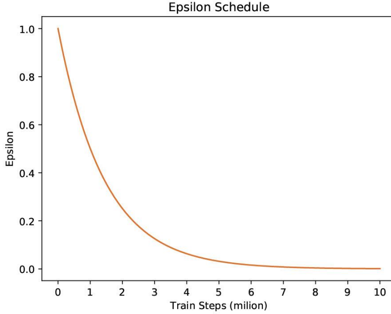
Fig. 2. Scheduling epsilon from 1 to 0.001 exponentially.
