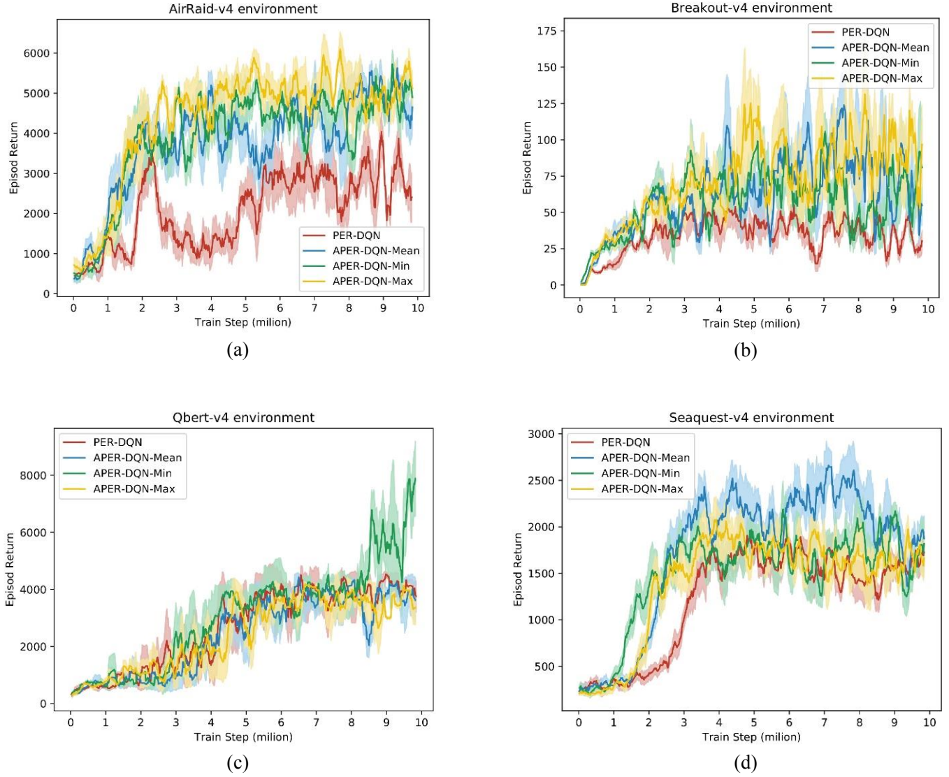
Fig. 4. Comparison of episode returns in DQN with prioritized experience replay (PER-DQN) and Adaptive prioritized experience replay (APER-DQN) using different aggregation functions.
