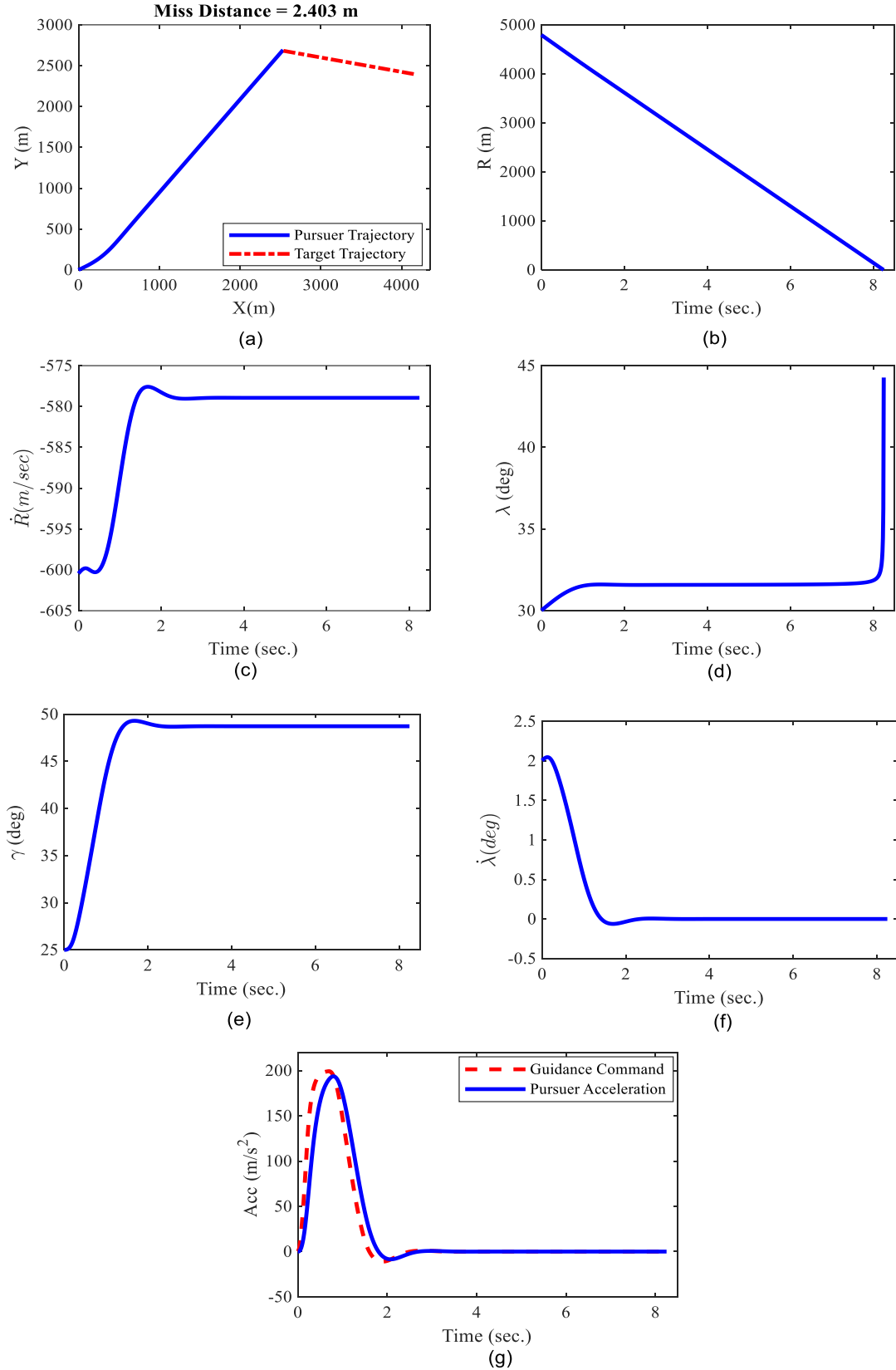
Fig. 4. Simulation Results for the Second Scenario: (a): Pursuer and target path; (b): The relative distance between the pursuer and the target; (c) The relative velocity between the pursuer and the target; (d) LOS angle; (e) Flight path angle of the pursuer; (f) LOS rate; (g) Guidance command and pursuer acceleration.
